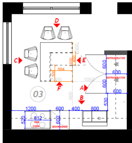
PLAN VIEW
